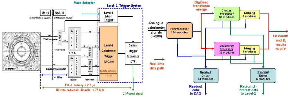
Figure 2.3: Overview: ATLAS Level-1 Trigger (a) and ATLAS Level-1 Calorimeter Trigger (b).
