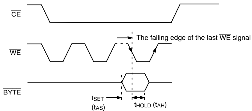
Figure 16. \overline{BYTE} Timing Diagram for Write Operations
