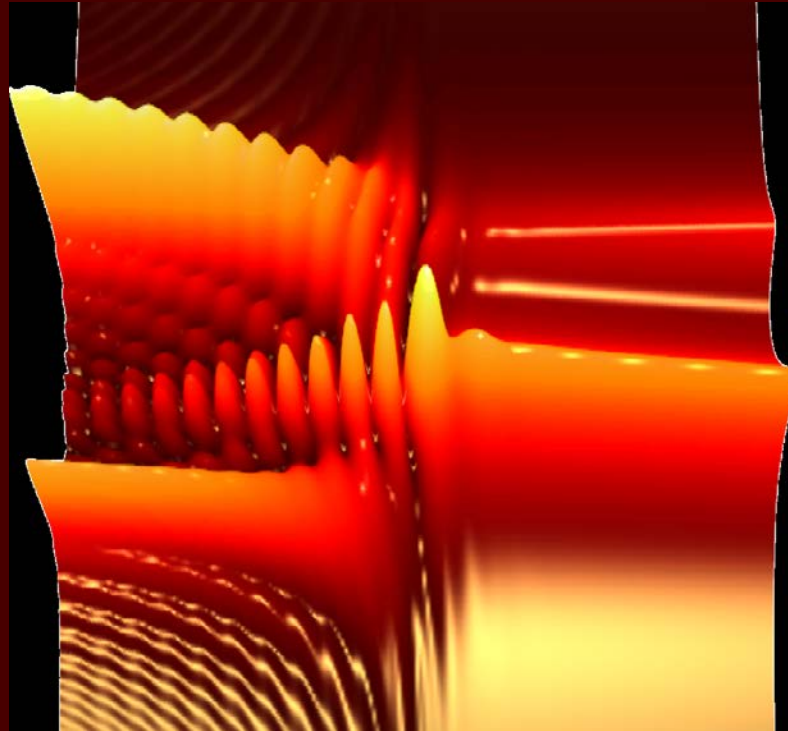
Time resolved pump-probe spectroscopy of polaritons in a microcavity
