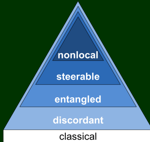
Hierarchy of quantum correlations
