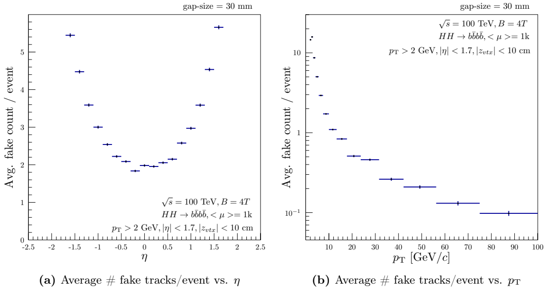
Figure 8.5: Average number of fake TTT tracks per event for the FCC-hh setup as a function of \eta (a) and p_T (b) using the HH \rightarrow b\bar{b}b\bar{b} signal sample in \langle \mu \rangle = 1k .
