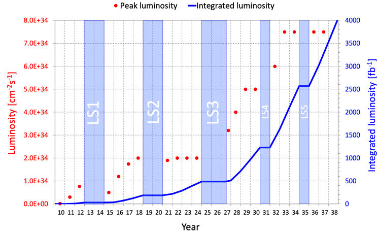
Figure 4.3: Instantaneous and integrated luminosities for Run1 and Run2 including projections for Run3 and the HL-LHC using the ultimate instantaneous luminosity at HL-LHC [81].
