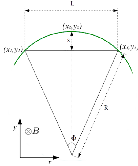
Figure B.1: A charged particles trajectory (green) passing through three detector layers in the transverse (x - y) plane. It makes three hits indicated as (x_i, y_i) , i = 1, 2, 3 when passing through a uniform magnetic field B perpendicular to the transverse plane.
