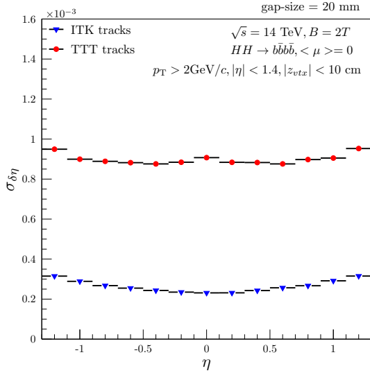
(e) \eta resolution vs. \eta
