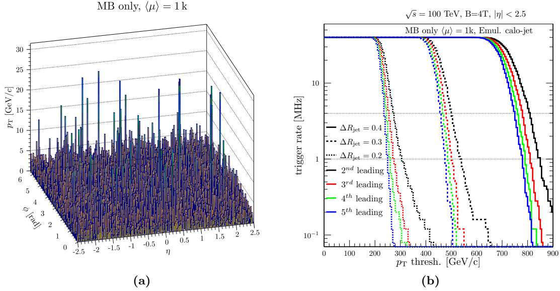
Figure 5.8: Transverse momentum recorded in the \eta - \phi cells for a minimum bias event with \langle\mu\rangle = 1\text{ k} (a) and trigger rate as a function of trigger threshold (b) using a calorimeter (with a granularity of \Delta\eta \times \Delta\phi = 0.01 \times 0.009 ) emulated at R_{\text{calo}} = 2\text{ m} for FCC-hh experiment.
