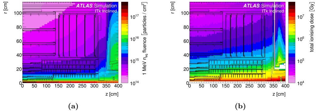
Figure 4.8: Simulated Non-Ionizing Energy Loss (NIEL) fluence (a) and Total Ionizing Dose (TID) (b) distributions for the ATLAS ITk layout for an integrated luminosity of 3000 \text{ fb}^{-1} [93].
