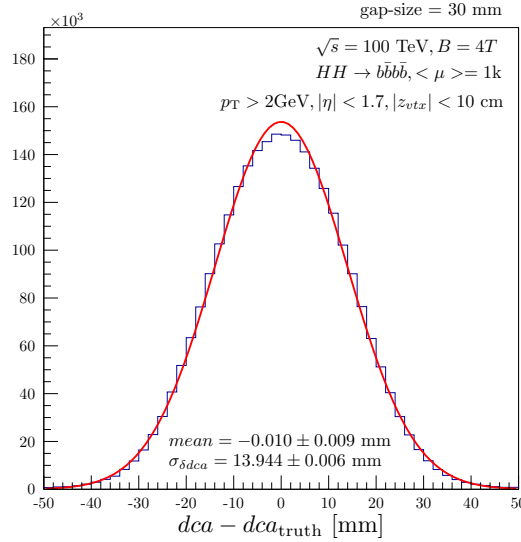
Figure 8.8: dca resolution of TTT tracks in the FCC-hh setup for the HH \rightarrow b\bar{b}b\bar{b} signal sample in \langle \mu \rangle = 1 \text{ k} .
