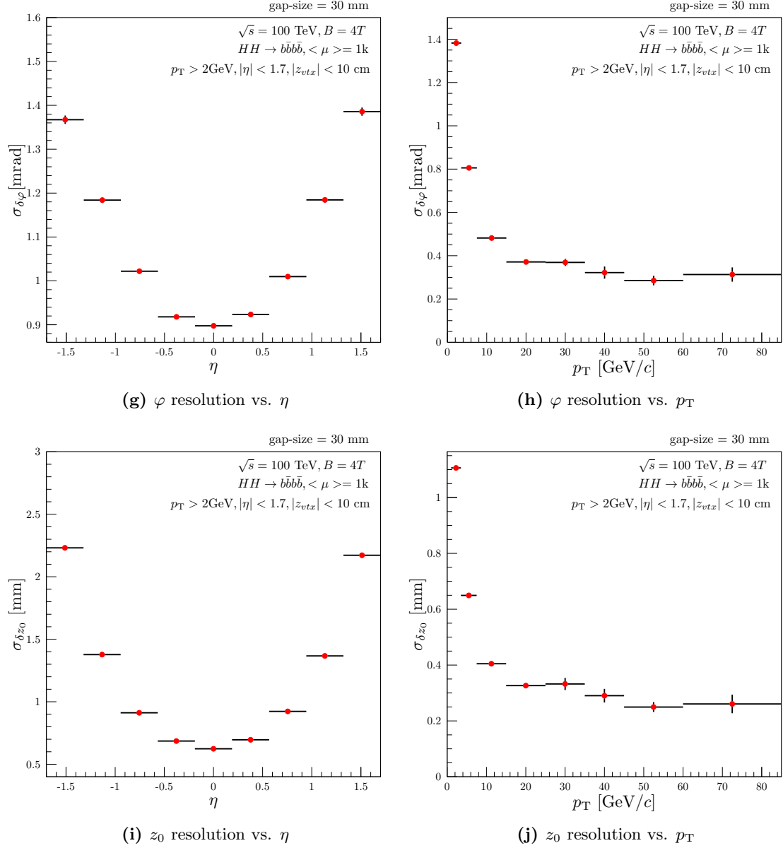
Figure 8.7: TTT Track parameter resolutions of relative p_T (a, b), inverse p_T (c, d), \eta (e, f), \varphi (g, h), and z_0 (i, j), in FCC-hh as a function of \eta (left) and p_T (right) using the HH \rightarrow b\bar{b}b\bar{b} signal sample in \langle \mu \rangle = 1 k.
