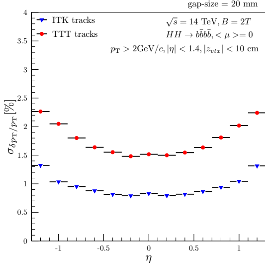
(a) relative p_T resolution vs. \eta
