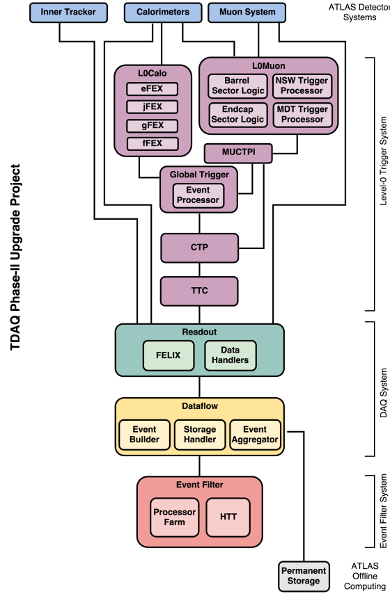
Figure 4.9: Functional block diagram of the baseline TDAQ Phase-II upgrade architecture, highlighting the three main sub-systems: Level-0 Trigger, DAQ, and Event Filter. Direct connections between each Level-0 trigger component and the readout system are suppressed for simplicity [69].
