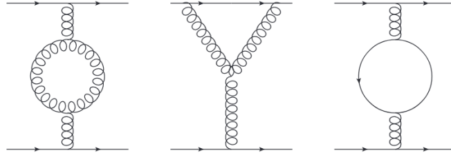
Figure 1.2: Feynman diagrams contributing to the renormalisation of the strong coupling.
