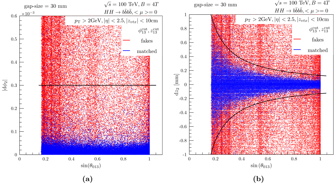
Figure 7.8: Control distributions to set the middle layer redundancy cuts \Delta\phi_2^{\text{cut}} and \Delta z_2^{\text{cut}} for the FCC-hh setup. Shown in the figures are the difference between the estimated and real: \phi_2 (a), and z_2 (b) as a function of sine of the reconstructed \theta .
