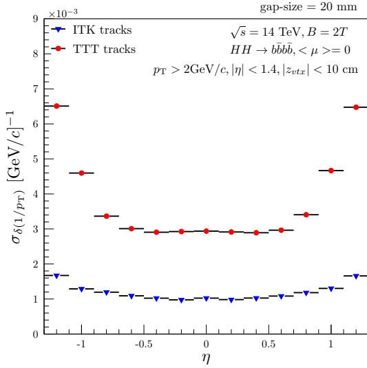
(c) inverse p_T resolution vs. \eta
