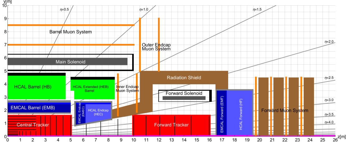
Figure 5.3: Layout of one quadrant of the FCC-hh reference detector along the y-z plane. Different sub-systems are indicated by various colours [41].
