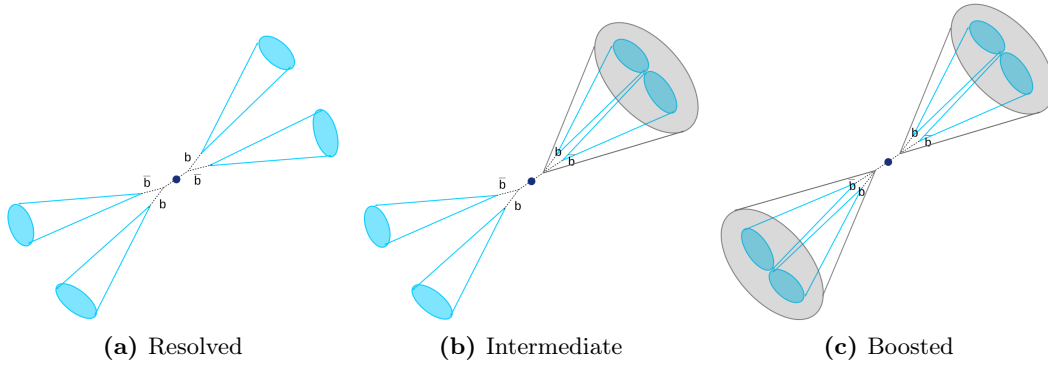
Figure 2.11: Illustration of resolved (a), intermediate (b), and boosted (c) category of final state b-jets in the HH \rightarrow b\bar{b}b\bar{b} physics channel.
