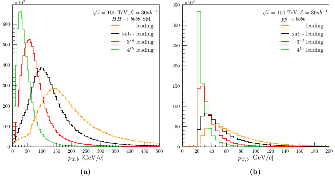
Figure 3.2: Transverse momentum of the four b quarks in: (a) HH \rightarrow b\bar{b}b\bar{b} process and (b) pp \rightarrow b\bar{b}b\bar{b} QCD multi-jet background after tracker acceptance cut of |\eta| < 2.5 .
