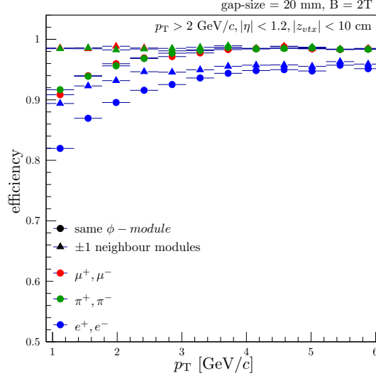
Figure 8.3: TTT track reconstruction efficiencies for single particles, namely, muons (red), pions (green), electrons (blue), illustrating the inefficiencies caused for p_T < \sim 4 \text{ GeV}/c by exclusion of the neighbouring \phi -modules during triplet hit selection.
