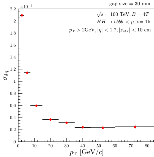
(f) \eta resolution vs. p_T
