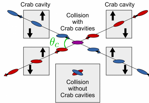
Figure 4.4: Depiction of beam manipulation using superconducting radio frequency (RF) crab cavities (CC) (the arrows indicate the torque on the bunch generated by the transverse RF field). Bunch collision at IP without CC is also shown. Figure adapted from [82].
