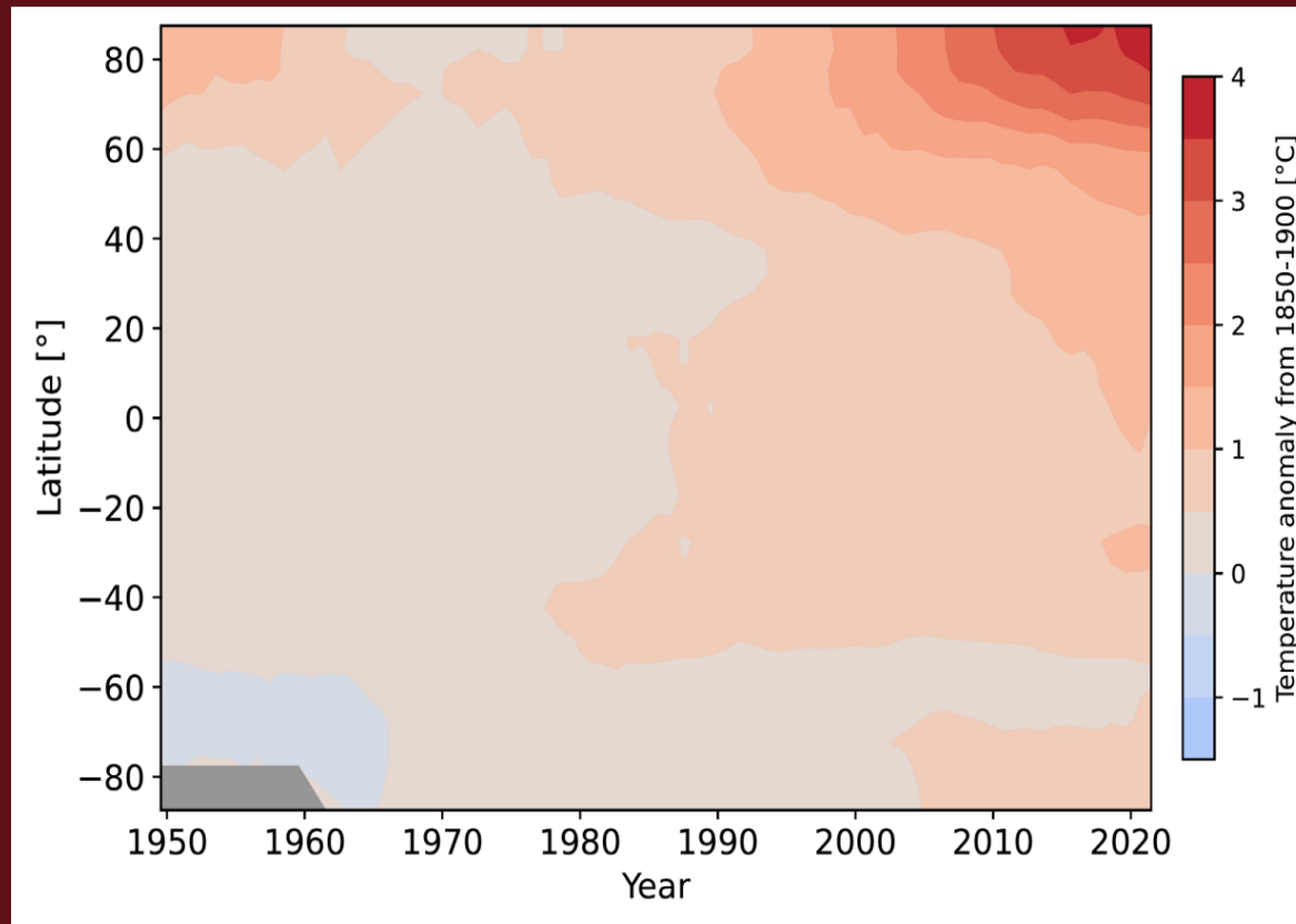
Pol-equator-pole, zonally averaged temperature anomaly (relative to the mean of 1850 to 1900) of the Earth's surface since the birth of physical climate modelling (Analysis by Christian Wirths, University of Bern).
