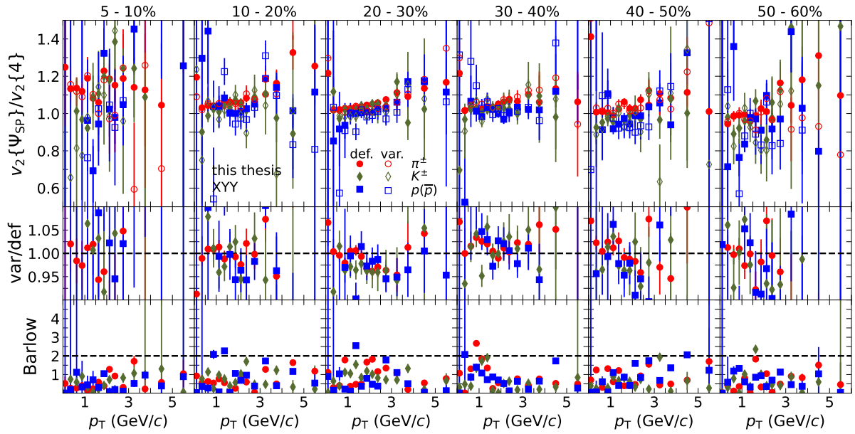
Figure 6.59: Comparison of the varied selection with the default selection for v_2\{\Psi_{SP}\}/v_2\{4\} for pions (red markers), kaons (green markers) and (anti)protons (blue markers) as a function of transverse momentum in all centrality intervals analyzed.
