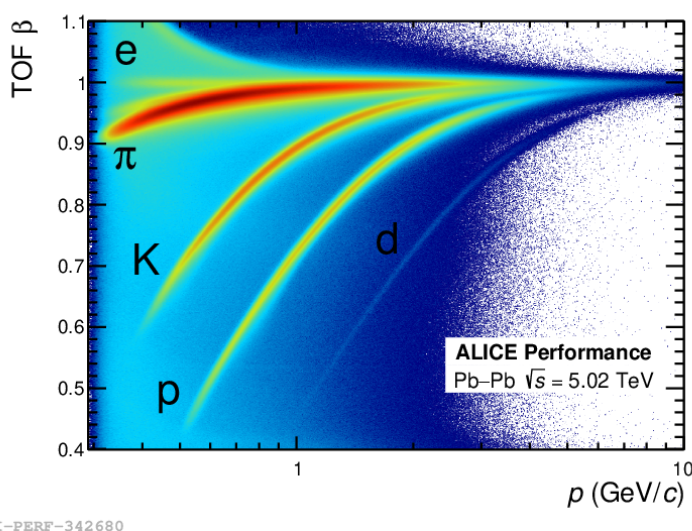
Figure 4.6: Velocity \beta measured by the TOF detector as a function of particle momentum in Pb–Pb collisions at \sqrt{s_{\text{NN}}} = 5.02 TeV. Wrongly associated tracks are seen outside of the particle bands [91].
