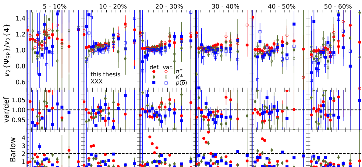
Figure 6.55: Comparison of the varied selection with the default selection for v_2\{\Psi_{SP}\} for pions (red markers), kaons (green markers) and (anti)protons (blue markers) as a function of transverse momentum in all centrality intervals analyzed.
