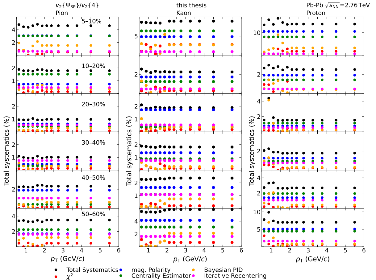
Figure 6.67: Total systematic uncertainties applied to the v_2\{\Psi_{SP}\}/v_2\{4\} of pions (left panels), kaons (middle panels) and (anti)protons (right panels) as a function of transverse momentum in all analyzed centrality intervals. The ZDC scale uncertainty of \approx 3\% is not shown in the figure.
