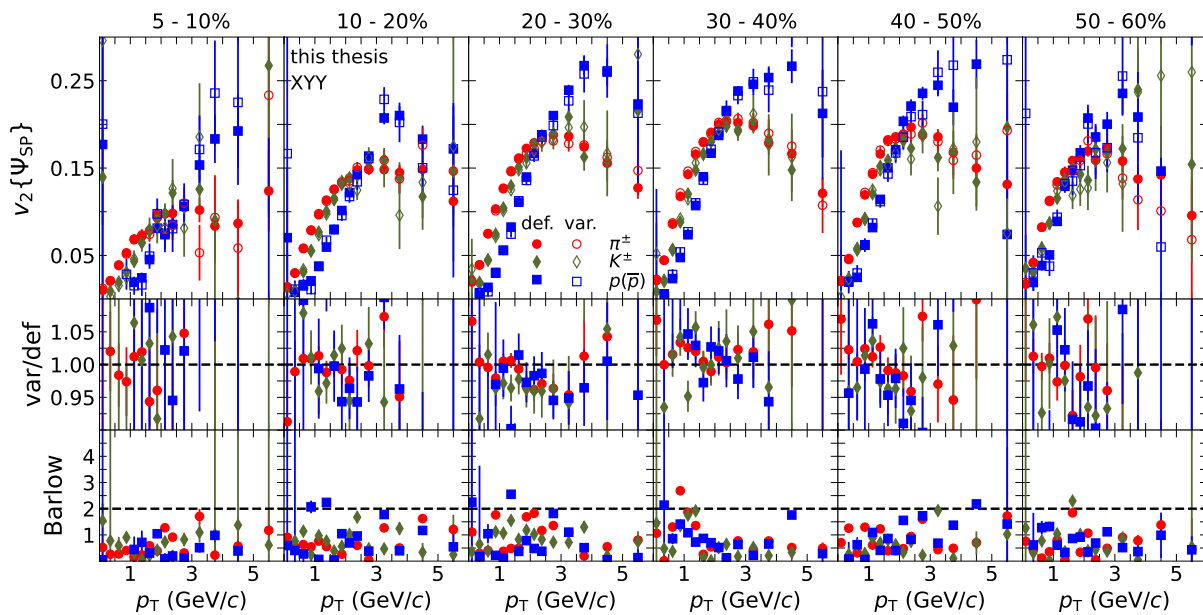
Figure 6.58: Comparison of the varied selection with the default selection for v_2\{\Psi_{SP}\} for pions (red markers), kaons (green markers) and (anti)protons (blue markers) as a function of transverse momentum in all centrality intervals analyzed.
