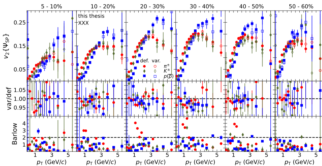
Figure 6.55: Comparison of the varied selection with the default selection for v_2\{\Psi_{SP}\} for pions (red markers), kaons (green markers) and (anti)protons (blue markers) as a function of transverse momentum in all centrality intervals analyzed.
