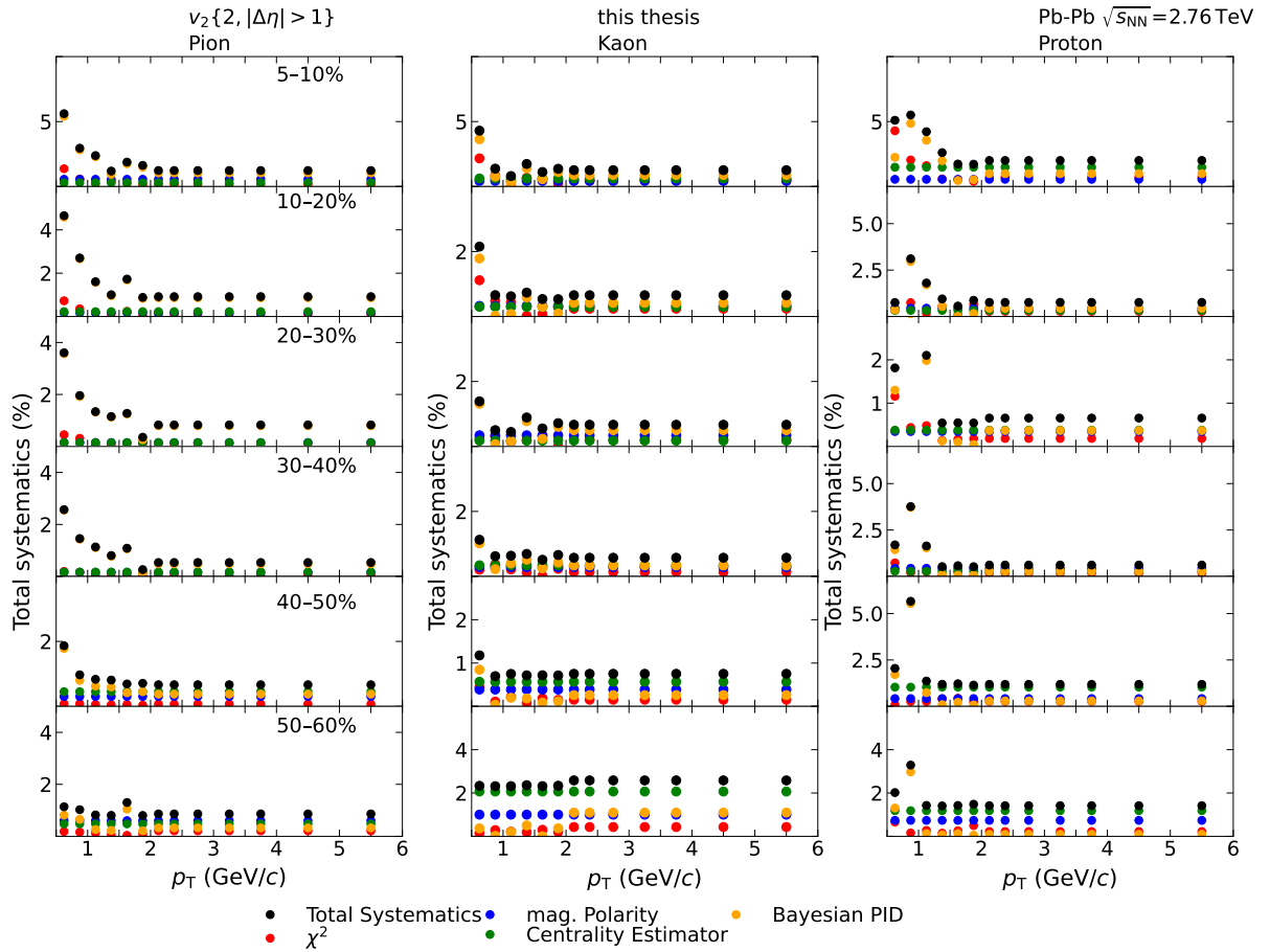
Figure 6.65: Total systematic uncertainties applied to the v_2 \{2, |\Delta\eta| > 1\} of pions (left panels), kaons (middle panels) and (anti)protons (right panels) as a function of transverse momentum in all analyzed centrality intervals.
