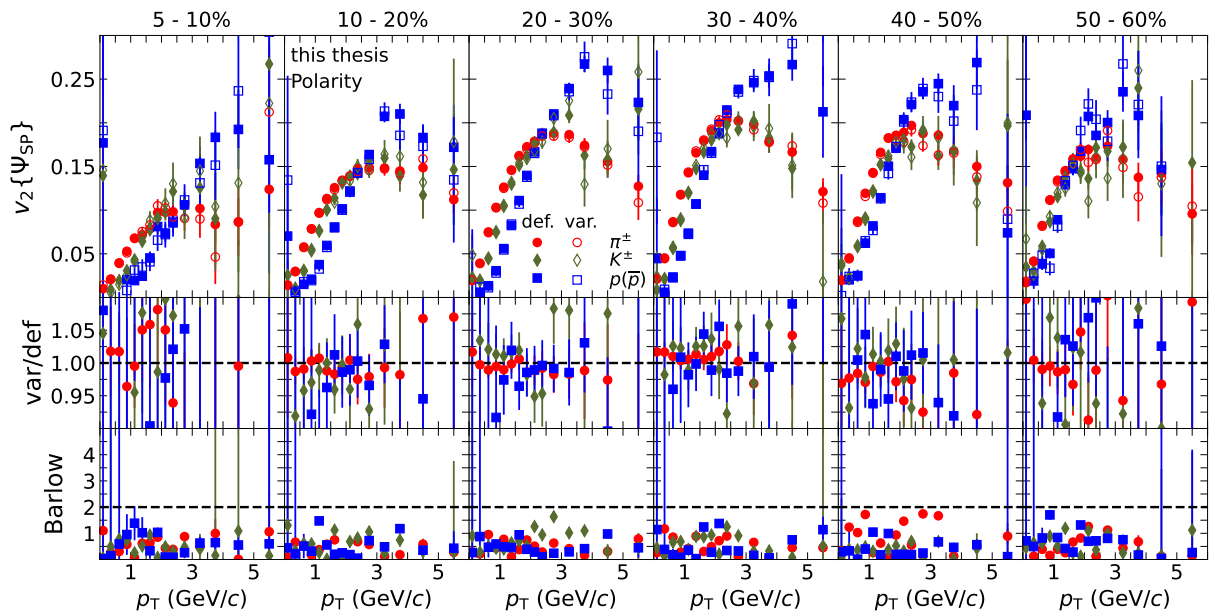
Figure 6.22: Comparison of the varied selection with the default selection for v_2\{\Psi_{SP}\} for pions (red markers), kaons (green markers) and (anti)protons (blue markers) as a function of transverse momentum in all centrality intervals analyzed.
