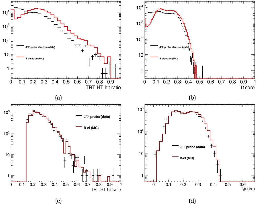
Figure 7.7: Electron distributions (a) TRT high threshold hit ratio distribution and (b) f_1(\text{core}) distribution showing the hadronic contamination at low values. The Monte Carlo is normalized to the entries in the data. The distributions (c) and (d) shows the TRT high threshold hit ratio and f_1(\text{core}) after removing the hadronic contamination.
