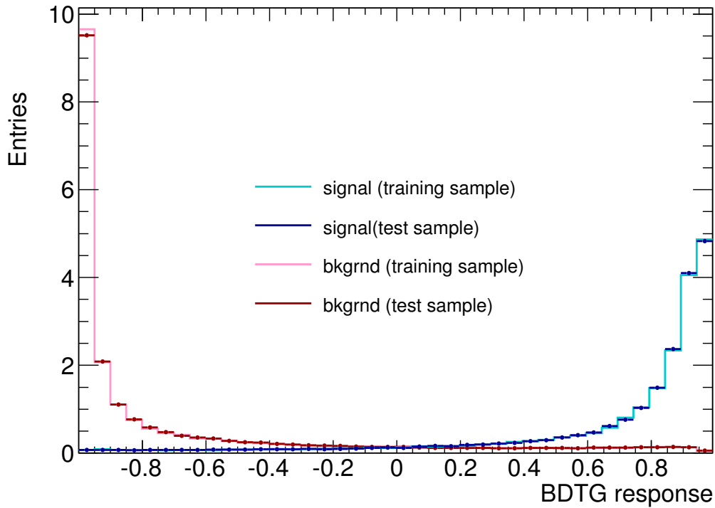
Figure 7.9: Overtraining check for BDTG classifier. A statistically independent sample is used to check if the classifier is overtrained. The plot shows that there is no significant overtraining
