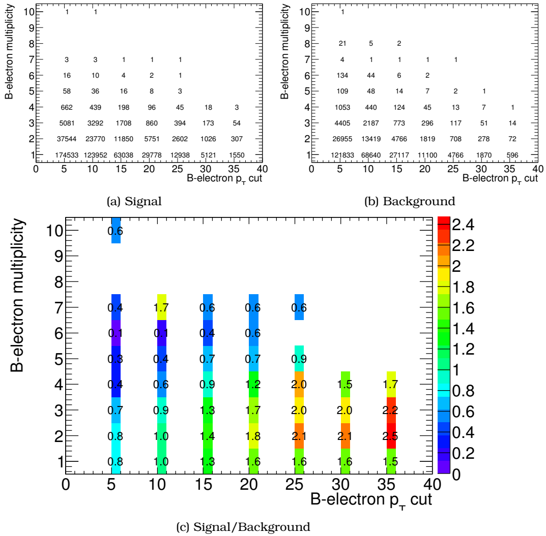
Figure 8.10: Truth Matched B-electron from (a) an exclusive signal sample ( Z \rightarrow e^+e^- + b\bar{b} \rightarrow e^+ + e^- ) and (b) Z +light jets background sample plotted as a function of low p_T cut in respective multiplicity bins. The B-electron contribution from Z + light jets sample is due to B-hadrons produced in parton shower. At low p_T such contaminations are present even in the Z + b\bar{b} sample. As we scan through from low p_T cut bins to high p_T cut bins, these soft component gets progressively removed. (c) shows the ratio of normalized (a) and (b). The signal to noise ratio increases as we scan through the p_T cut bins
