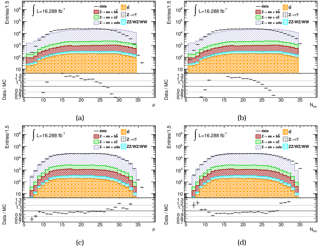
Figure 8.1: (a) and (b) show the average number of interactions per proton bunch crossing and number of primary vertices reconstructed in an event respectively using default settings. Both variables are a measure of pileup. (c) and (d) show the same variables after applying weights to the Monte Carlo samples. After re-weighting, the Monte Carlo agreement with data improves significantly.
