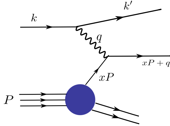
Figure 3.1: Schematic representation of Deep Inelastic scattering. An electron with momentum k interacts with hadron with momentum P
