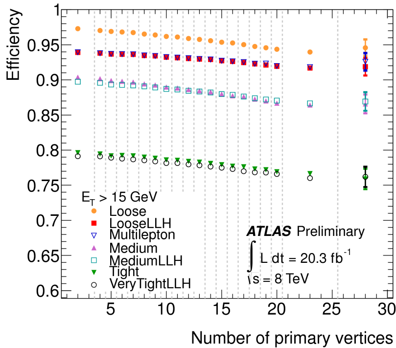
Figure 6.15: Measured reconstruction efficiency for various electron selection menus, as a function of number of primary vertices. The menus are relatively stable to pileup [41]
