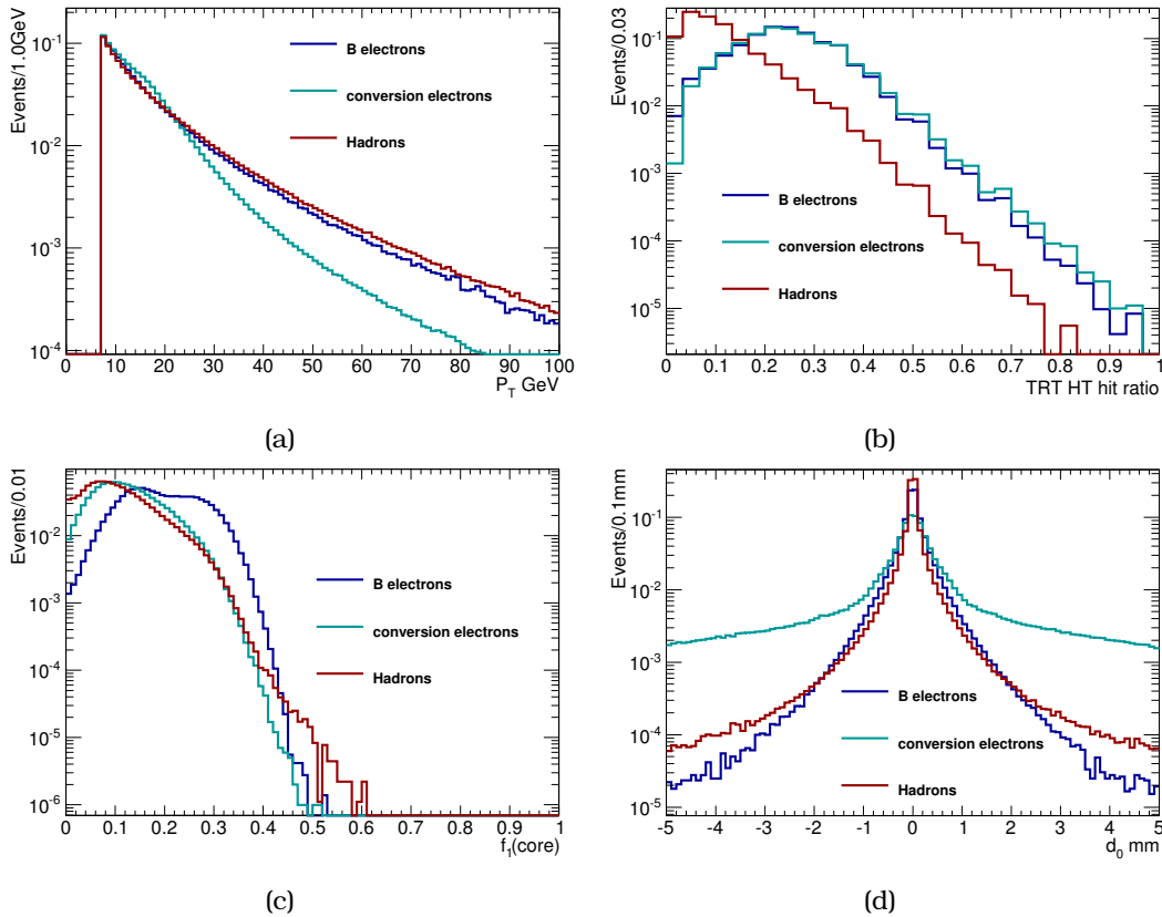
Figure 7.3: Normalized distributions of signal electrons (B electrons) and electrons from photon conversions and hadrons in (a) p_T (b) in TRT high threshold hit ratio (c) f_1(\text{core}) (d) d_0 , the transverse impact parameter
