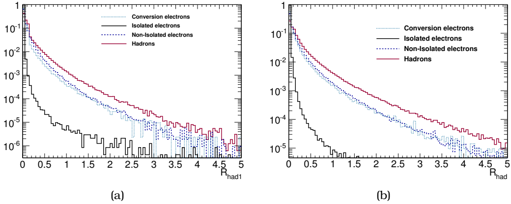
Figure 6.3: Energy leakage into the hadronic calorimeter parameterized as (a) R_{had1} : Ratio of energy deposited in the first layer of the hadronic calorimeter to the energy deposited in the electron cluster (b) R_{had} : Ratio of energy deposited in all hadronic layers to the energy deposited in the electron cluster.
