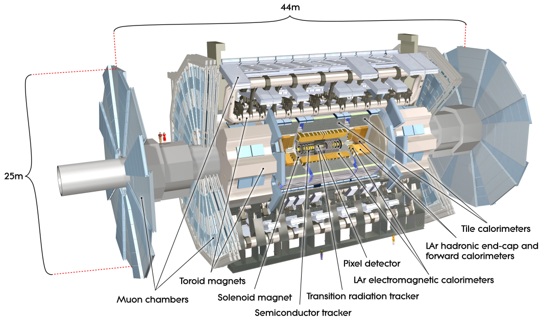
Figure 4.3: Cut away view of the ATLAS detector. A cartoon of two human beings are also included to highlight the size of the detector
