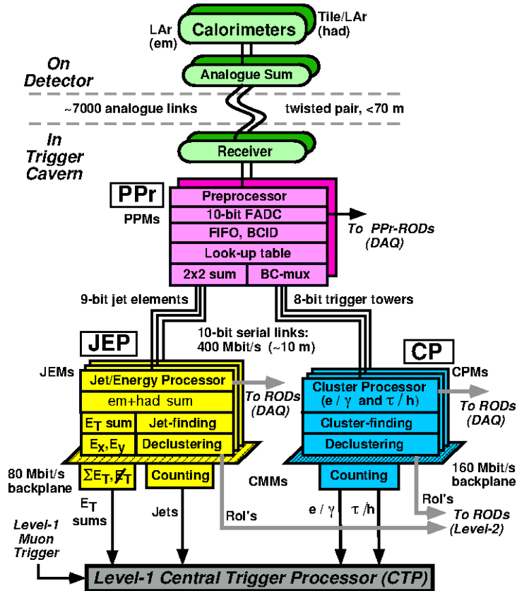
Figure 5.1: A schematic representation of the L1Calo trigger system. Black arrows show real time data path, and grey arrows show readout data path [36]
