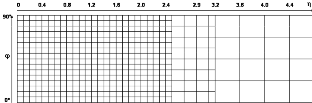
Figure 5.3: Trigger tower granularity in \eta and \phi [36]
