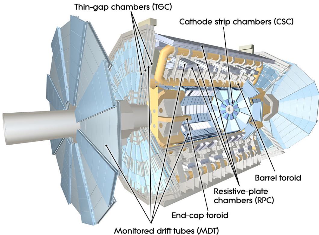
Figure 4.8: The ATLAS muon spectrometer
