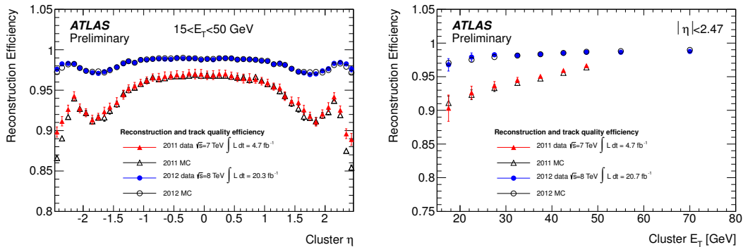
Figure 6.2: Electron reconstruction efficiency as a function of (a) cluster \eta and (b) cluster E_T . The red curve represent 2011 data and the blue curve represent 2012 data [41]
