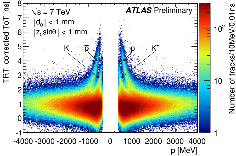
Figure 4.5: Time over threshold estimator showing particle identification capabilities of the TRT as a function of momentum
