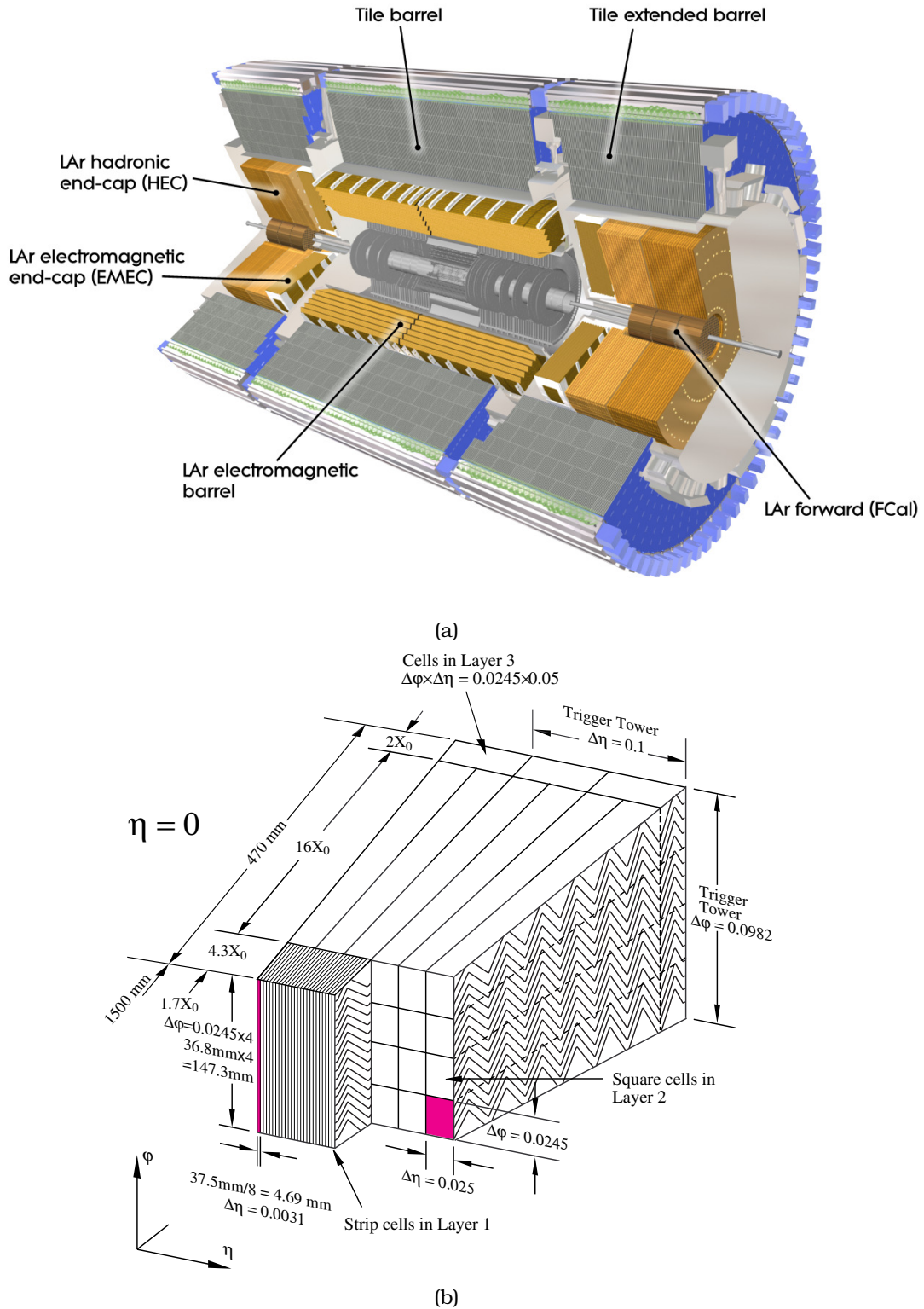
Figure 4.7: (a) Cut away view of the ATLAS calorimeter system (b) Sketch of a LAr barrel module showing different calorimeter layers with varying granularity in each layers.
