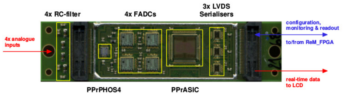
Figure 5.5: PreProcessor Multi-Chip Module: The FADCs convert the analog input signals to digital signals [37].
