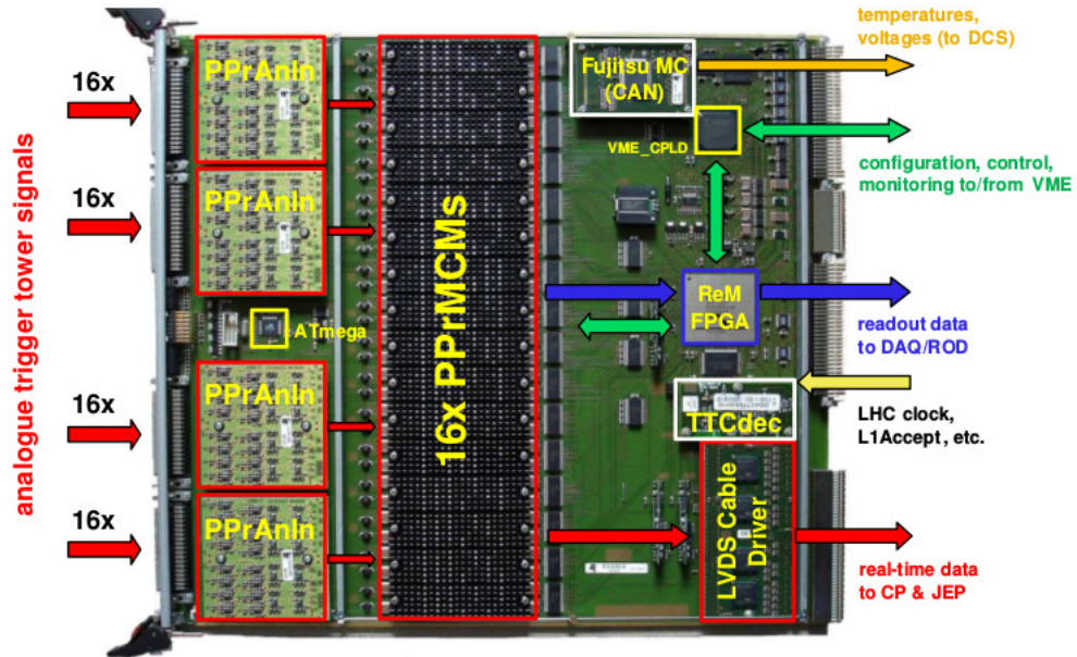
Figure 5.4: The Preprocessor module [37]
