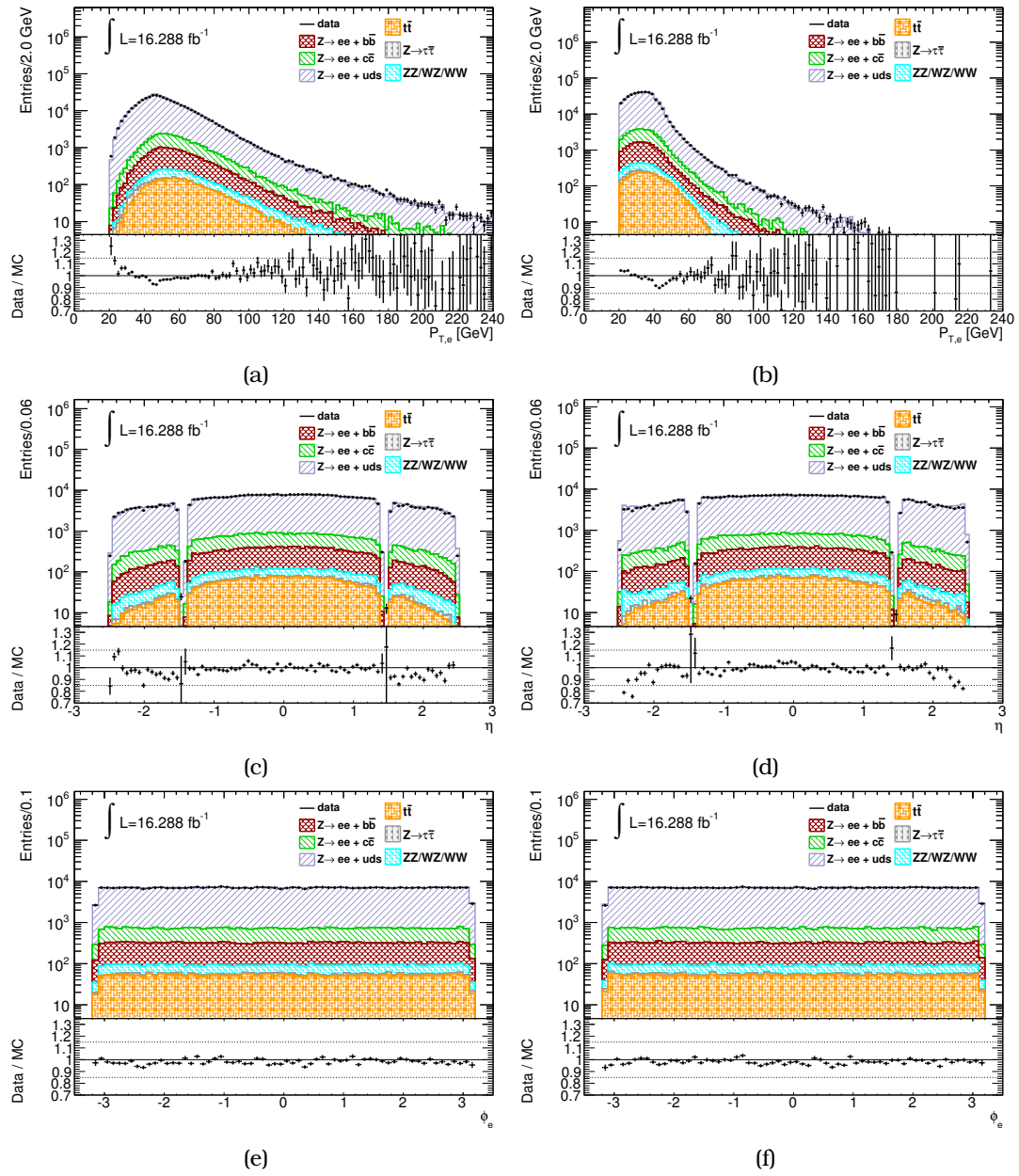
Figure 8.4: p_T , \eta and \phi control distributions for electrons which pass medium++ identification cuts. The plots on the right and left are the distributions for the leading p_T and the subleading p_T electron
