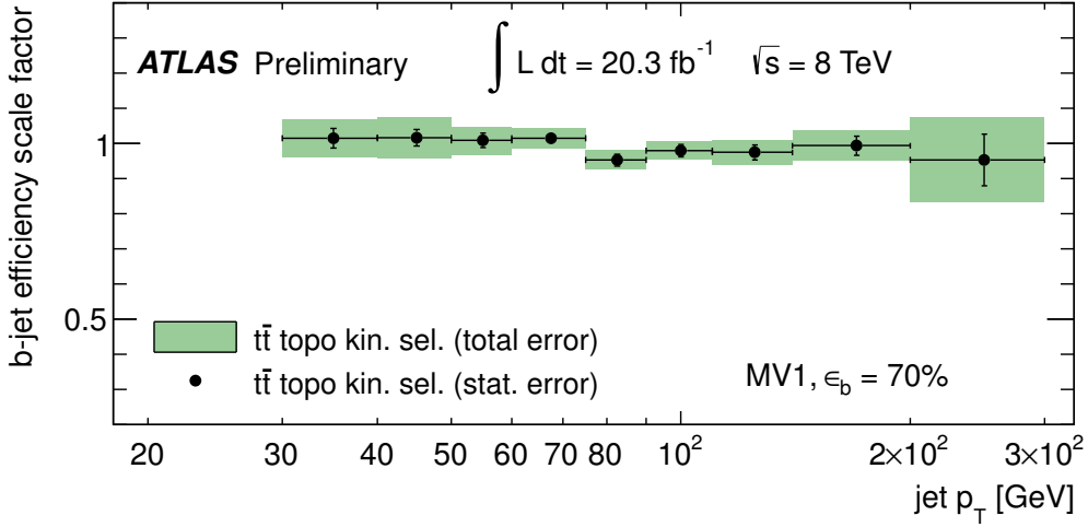
Figure 7.1: B-tagging efficiency scale factor and uncertainties shown as a function of jet p_T for the MV1 b-jet tagger. The uncertainties on the scale factors range from 6% to 8% [46]
