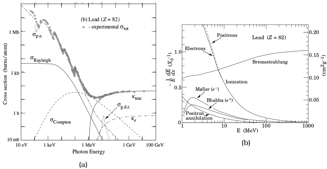
Figure 4.6: Cross sections for various interactions with matter for (a) photons and (b) electrons and positrons [32]
