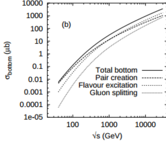
Figure 8.9: Total bottom cross section for pp collisions as a function of center of mass energy \sqrt{s} . The contribution from gluon splitting becomes substantial at the LHC energies [61]
