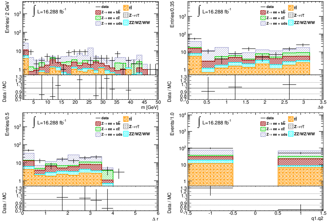
Figure 8.8: Charge combinations and angular separation distribution for non-Z electron candidates which pass a cut of 0.5 on soft electron response distribution
