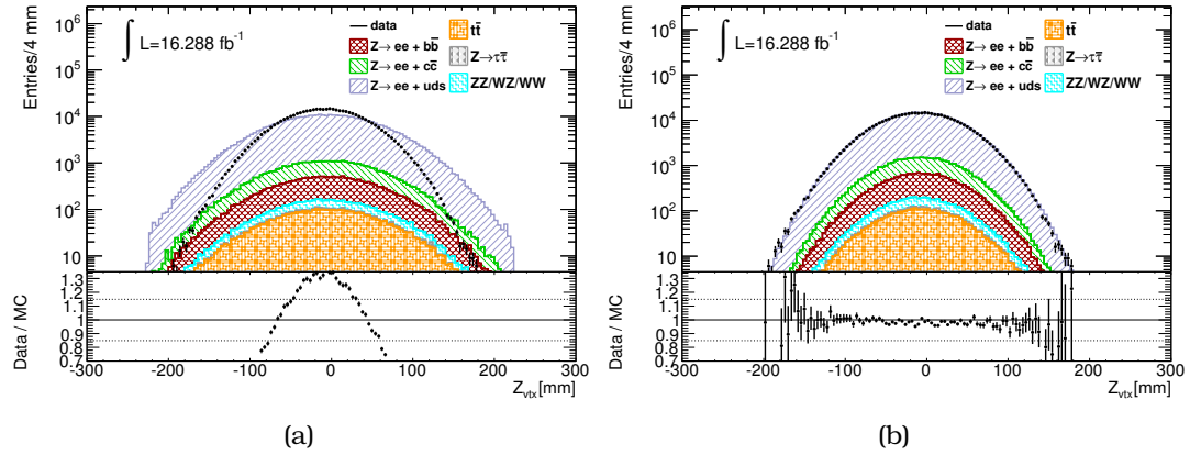
Figure 8.2: (a) The distribution of primary vertex z -coordinate in data and simulation (b) Primary vertex z -coordinate distribution after applying a weighting factor to the Monte Carlo samples to correct for this effect
