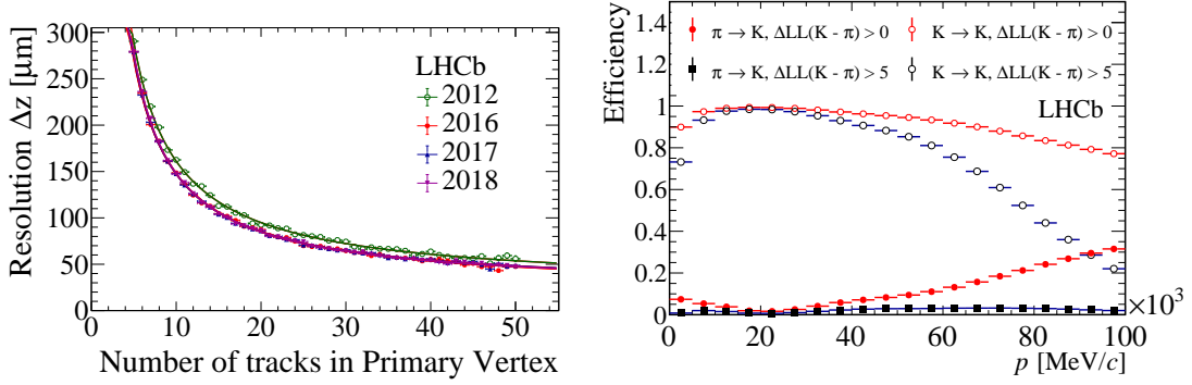
Figure 9.2: Left: Resolution of the PV reconstruction in z -direction. Right: Efficiency to select kaons and rate of pions misclassified as kaons for different PID requirements, with \Delta \text{LL}(K - \pi) = \Delta \ln \mathcal{L}_{K\pi} . Figures taken from [213].
