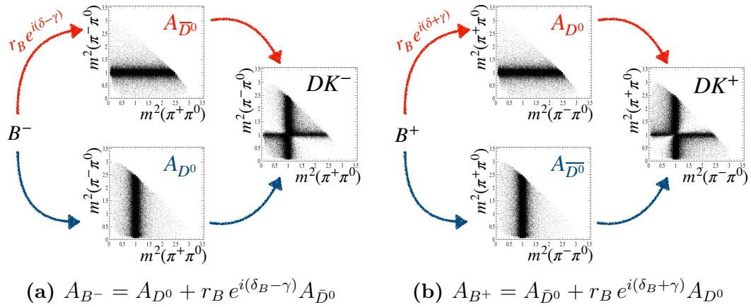
Figure 3.3: Superposition of decay paths contributing to the B^- \rightarrow DK^- (left) and B^+ \rightarrow DK^+ (right) processes with D \rightarrow \pi^+ \pi^- \pi^0 . The contribution of a single scalar resonance, R^\pm , is shown: D^0 \rightarrow (R^+ \rightarrow \pi^+ \pi^0) \pi^- and \bar{D}^0 \rightarrow (R^- \rightarrow \pi^- \pi^0) \pi^+ . The weak phase difference introduces an asymmetric interference pattern for the B^- and B^+ Dalitz plots. The values r_B = 0.5 , \delta_B = 70^\circ and \gamma = 70^\circ are chosen. Note that the axes on the B^+ Dalitz plots are flipped, i.e. CP -conjugated, with respect to the B^- Dalitz plot. In that case the visible phase-space structure of both coincides in case of no CP violation ( \gamma = 0 ).
