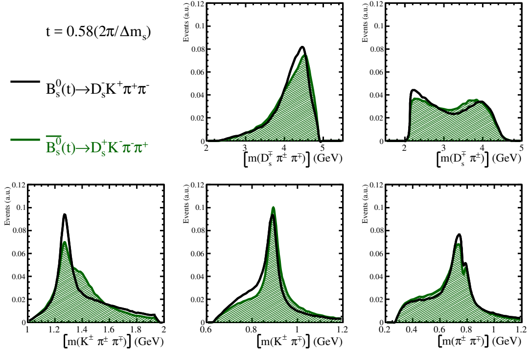
(b) Phase-space projections at decay time t = 0.58(2\pi/\Delta m_s) .
