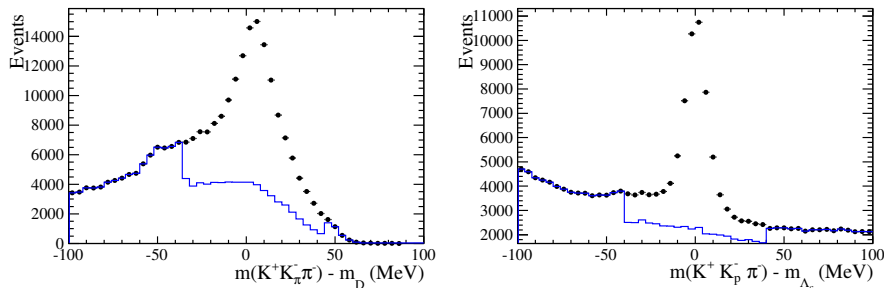
Figure 9.5: Background contributions to B_s \rightarrow (D_s^- \rightarrow K^+K^-\pi^-)\pi\pi\pi candidates originating from D^- decays where the \pi^- is misidentified as K^- (left) or from \Lambda_c^- decays where the \bar{p} is misidentified as K^- (right). The D_s invariant mass is recomputed applying a different mass hypothesis to the K^- candidate. The distributions are shown without (black) and with (blue) the veto cuts applied.
