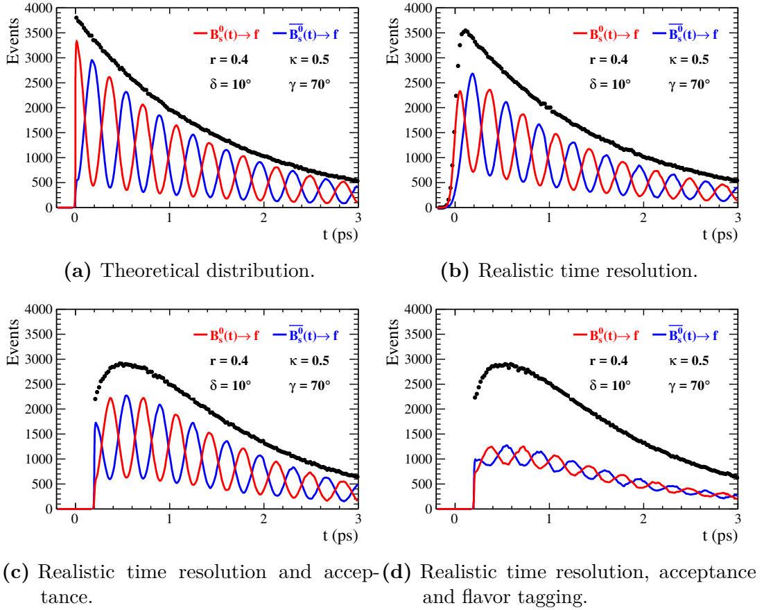
Figure 10.1: Illustration of various experimental effects on the decay rate.
