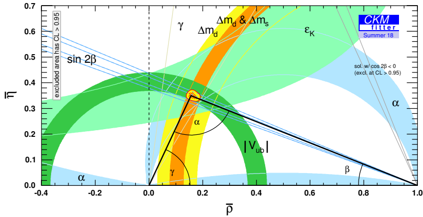
Figure 3.1: Current constraints on the CKM Unitarity Triangle [30]. The side V_{cd}V_{cb}^* is normalized to unit length. Constraints from the CKM angles \alpha , \beta and \gamma as well as from \Delta m_d and \Delta m_s and \epsilon_K are displayed (shaded areas). The red (yellow) area indicates the 68% (95%) confidence level region of the apex of the triangle.
