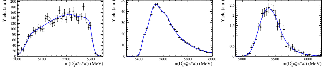
Figure 9.7: Left: Invariant-mass distribution of simulated B_s^0 \rightarrow D_s^* \pi \pi \pi decays, where the \gamma/\pi^0 from the D_s^* decay is excluded from the reconstruction. Middle: Invariant-mass distribution of simulated B_s^0 \rightarrow D_s \pi \pi \pi decays, where one of the pions is reconstructed as a kaon. Right: Invariant-mass distribution of simulated B_s^0 \rightarrow D_s^* \pi \pi \pi decays, where the \gamma/\pi^0 from the D_s^* decay is excluded from reconstruction and one of the pions is reconstructed as a kaon. Empirical models describing the shapes are shown in blue.
