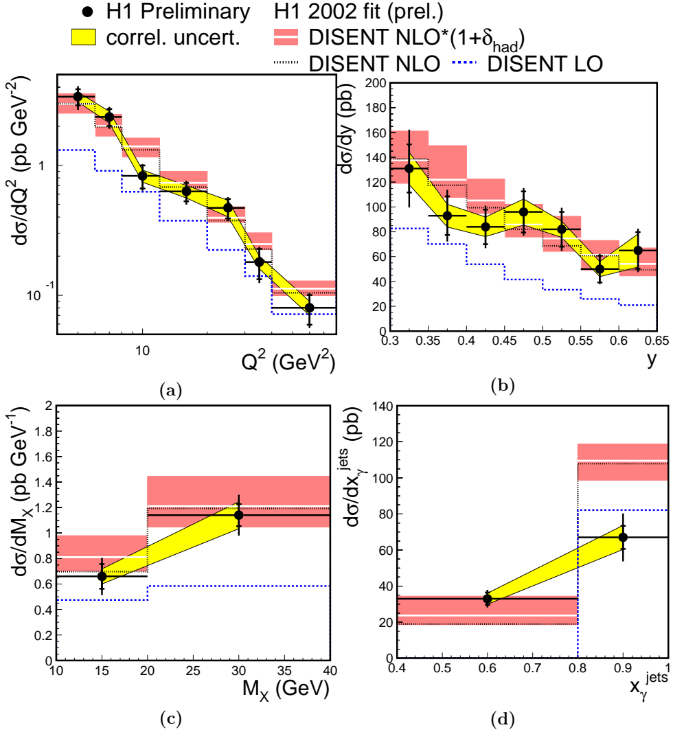
Figure 6: Cross section for the diffractive production of two jets in the DIS kinematic region specified in Table 1 as a function of the variables a) Q^2 , b) y , c) M_X and d) x_\gamma^{jets} . Also shown is the DISENT prediction based on the ‘H1 2002 fit’ diffractive PDFs at NLO with and without hadronisation corrections and at LO without hadronisation corrections. For details see the caption of Figure 4.
